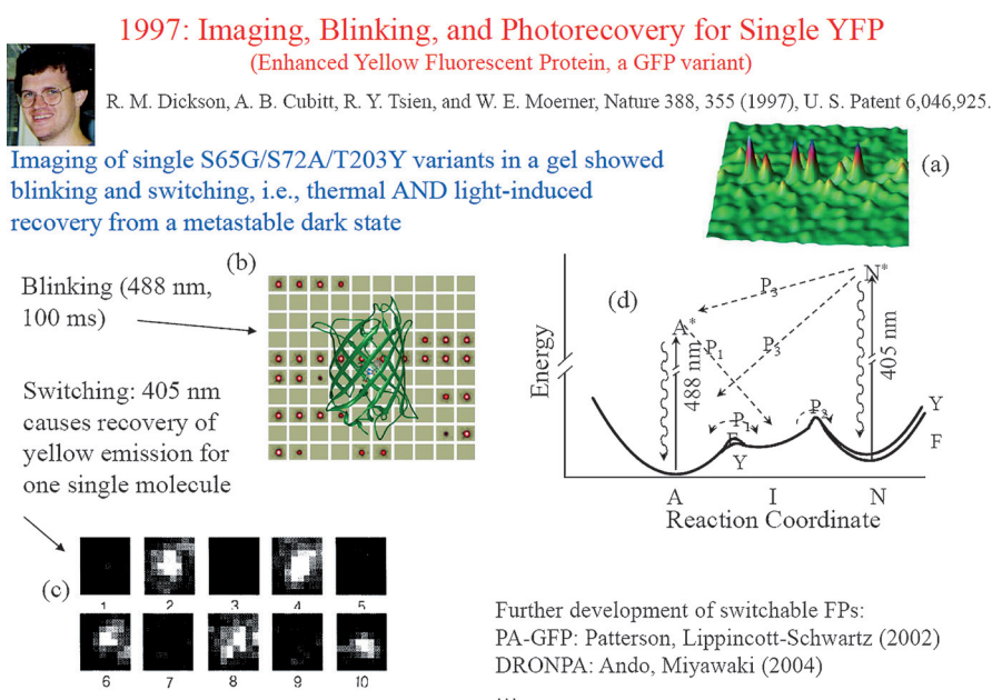
Figure 16. a) Imaging, b) blinking, and c, d) light-induced photorecovery or switching for single YFP. Photo: Rob Dickson. From Ref. [2].
