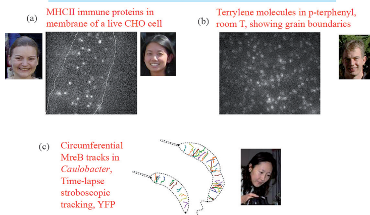
Figure 14. Selected single-molecule imaging and tracking studies at room temperature. From Refs. [158] (a), [104] (b), [108] (c). Photos left to right: Marija Vrljic, Stefanie Nishimura, Christopher (Kit) Werley, So Yeon Kim.
