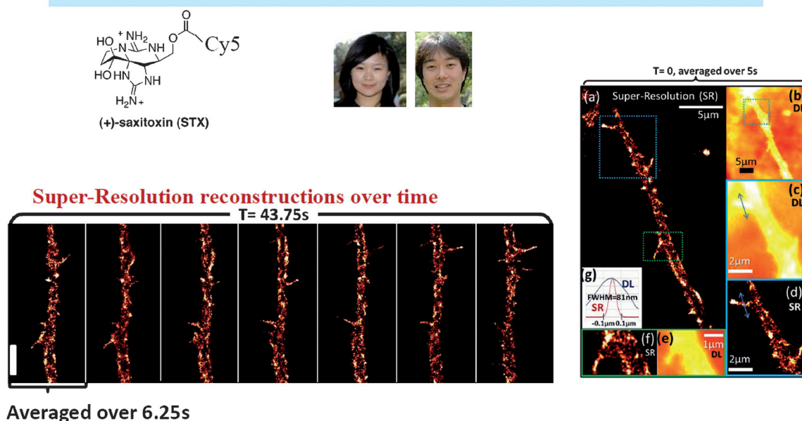
Figure 20. Example of super-resolution cellular imaging using a fluorescent saxitoxin ligand binding to ion channels on the cell surface. Bar in left sequence: 5 \mu\text{m} . From Ref. [168]. Photos: Hsiao-lu Lee, Shigeki Iwanaga.
