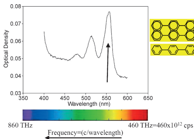
Figure 1. Spectrum (absorption versus wavelength, or color) of terrylene molecules in a solid host of p -terphenyl at room temperature.
