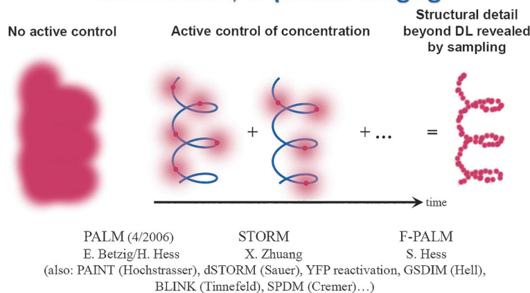
Figure 17. Active control of emitting concentration leads to super-resolution microscopy. From Ref. [155].
