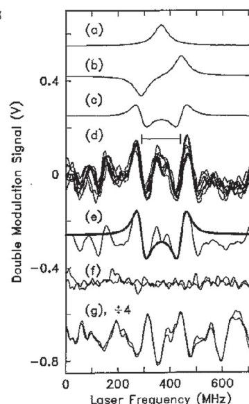
Figure 8. First optical detection and spectroscopy of single molecules in condensed matter. a–c) Buildup of expected lineshape for FM-Stark spectroscopy. d) Multiple scans showing a single molecule at 592.423 nm. e) Averaged scans compared to lineshape. f) Far into the wings of the line, no molecule. g) Closer to the center of the inhomogeneous line; SFS. Photo: Lothar Kador. From Ref. [1].
