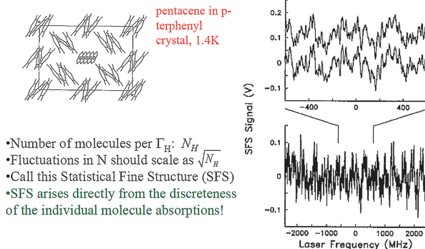
Figure 6. Observation of statistical fine structure (SFS) (right) for pentacene in p -terphenyl (schematic structure) with Tom Carter (photo). Data from Ref. [28].
