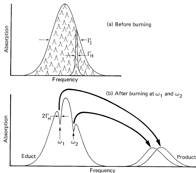
Figure 4. Illustration of persistent spectral hole-burning in inhomogeneously broadened lines of dopants in solids at low temperatures. a) Before burning, the inhomogeneously broadened line has a “smooth” absorption profile. b) When a narrowband laser irradiates selected frequencies in certain materials, spectral dips or “holes” can be generated.
