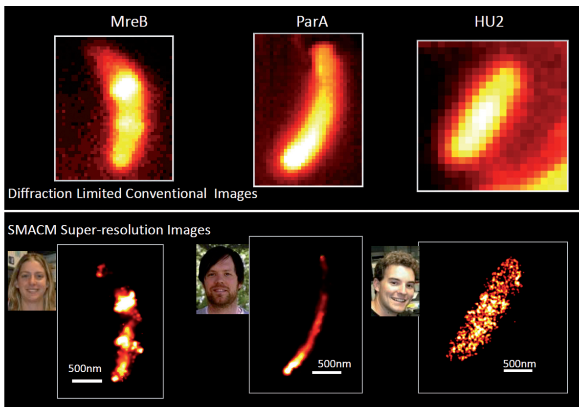
Figure 19. Super-resolution imaging of three different proteins in Caulobacter : MreB, [149] ParA, [163] HU2. [164] Photos left to right: Julie Biteen, Stephen Lee, Mike Thompson.
