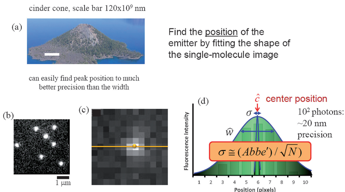
Figure 15. The central concepts behind super-localization of single-molecule emitters.
