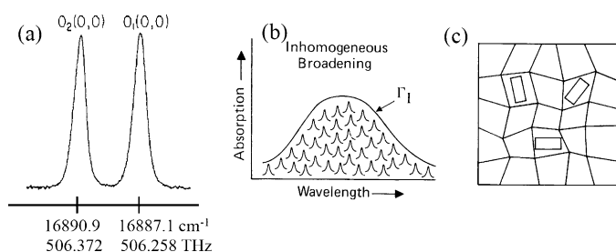
Figure 3. Inhomogeneous broadening in solids at low temperatures. a) Pentacene in p -terphenyl absorption spectra taken from Ref. [11] ( 0.09\text{ cm}^{-1} resolution). b) Schematic of the inhomogeneous broadening effect with width \Gamma_I . c) Schematic of different local environments giving rise to inhomogeneous broadening.
