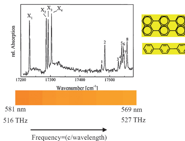
Figure 2. Spectrum (absorption versus frequency, wavenumber, or color) of terrylene molecules in a solid host, p -terphenyl, at low temperature ( \approx 2 K), from Ref. [10b].
