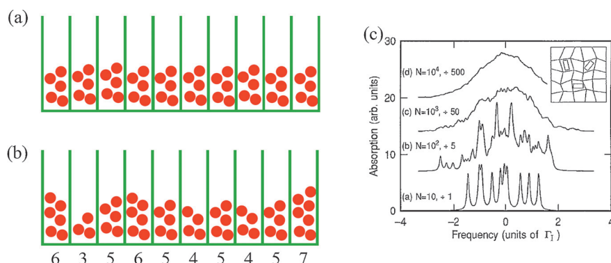
Figure 5. Illustration of number fluctuations for probability and for spectroscopy. a) An unlikely way to randomly throw 50 balls at 10 bins. b) A more likely case. c) Simulation of an inhomogeneously broadened line in a sample for the case of uniform Gaussian probability of selecting absorption frequencies.
