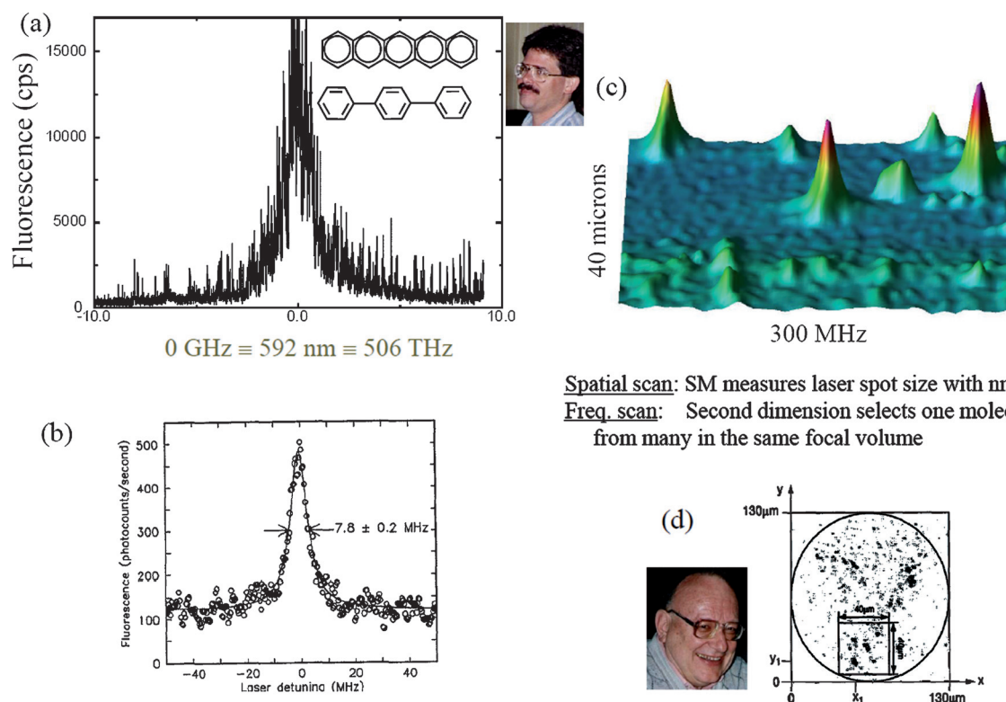
Figure 10. a, b) Single-molecule spectroscopy and c, d) imaging. Photos: W. Pat Ambrose (upper), Urs P. Wild. From Refs. [49] (a), [56] (b), [48] (c), [58] (d).
