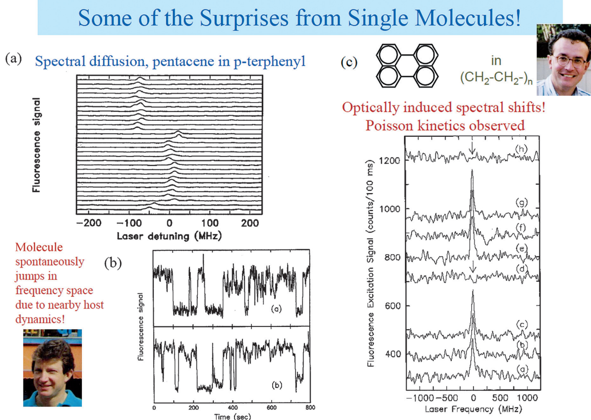
Figure 11. a, b) Spectral diffusion and c) light-induced spectral shifts. From Refs. [48, 56, 64], respectively. Photos: left: Jim Skinner, right: Thomas Basché.
