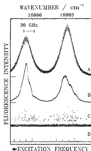
Figure 9. Single-molecule detection and absorption spectroscopy by recording the emitted fluorescence. A, B) The inhomogeneous line, C) at very low concentration; the dots represent the increases in emission when single molecules come into resonance with the tunable laser. Photo: Michel Orrit. From Ref. [35].
